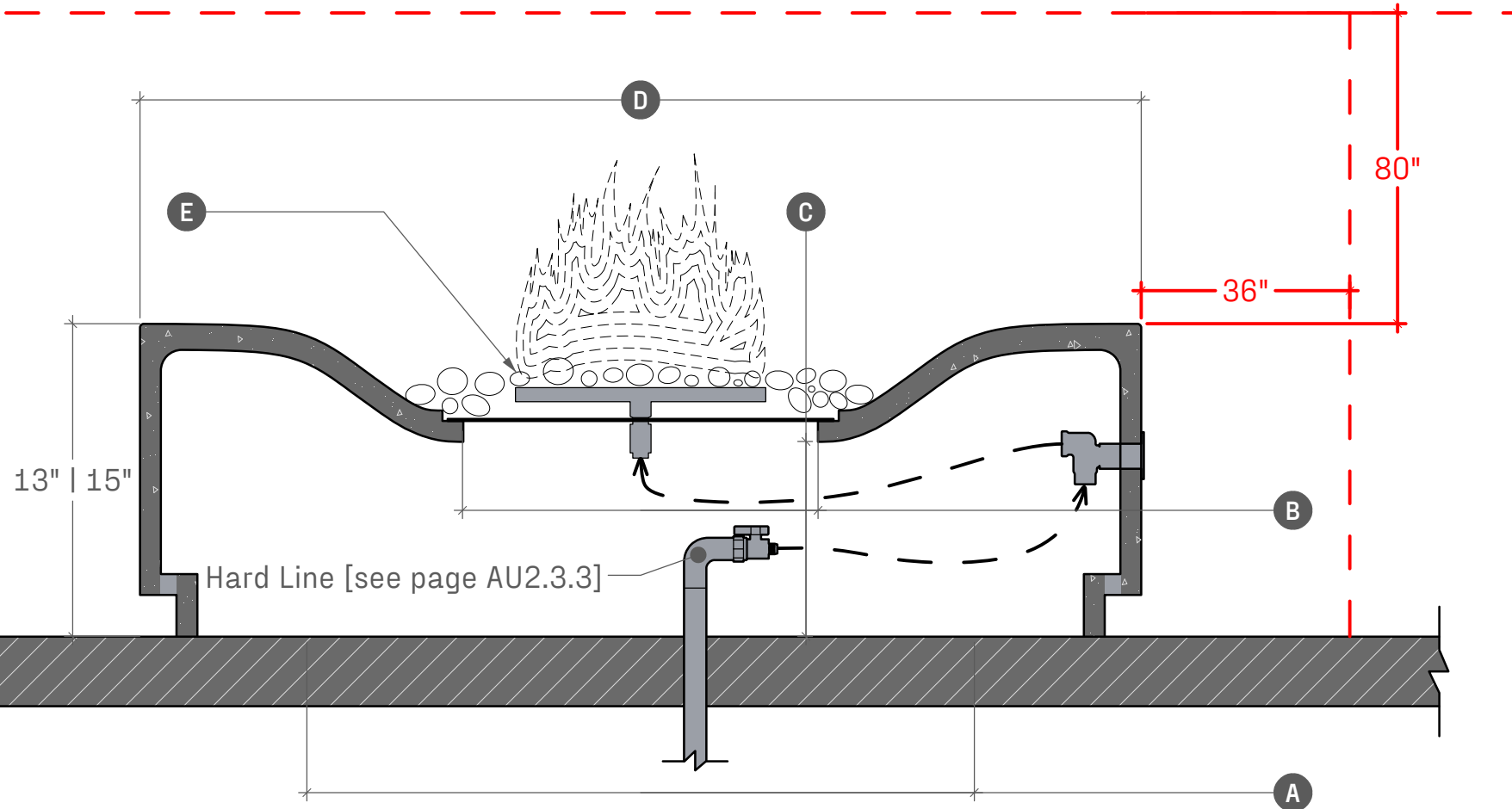
AU2.2.1 SECTION DETAIL SCALE: 1" = 0' - 8"
