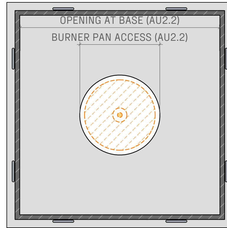
AU2.3.2 PLAN VIEW SCALE: 1" = 1' - 0"
